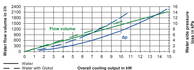
Water flow volume und water side pressure loss
